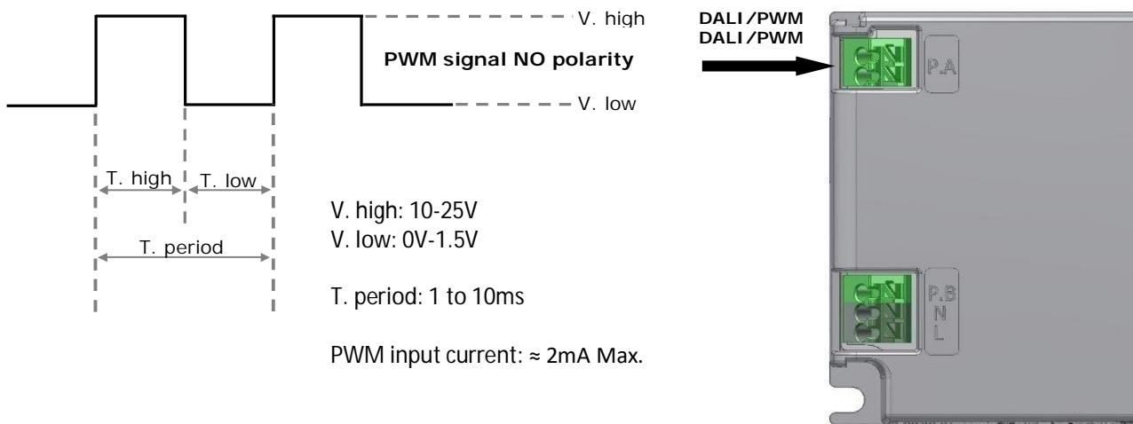
Figure 4: Ozone as PWM dimmable LED driver
