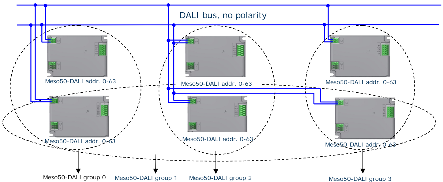
Figure 1: Ozone-DALI network (example connection)
